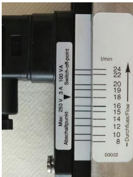
Fig. 4: Switch point adjustment scale DKM-1
