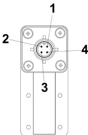
Fig 17 Pin-assignment, socket M12x1 Form 30x70)
