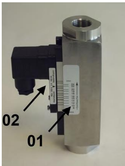
Fig. 1 DKM-1 flow monitor 01 Switch point adjustment scale 02 Switch contact with female socket or sealed-in cable
