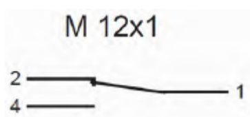
Fig. 20: Switch position under no-flow condition
