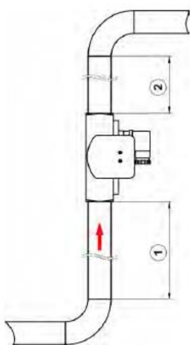
Fig. 7: Unimpeded flow sections
