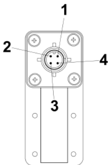
Fig. 18: Pin-assignment, socket M12x1 Form 30x70)
