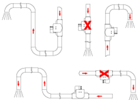
Fig. 8: Unimpeded outlet
