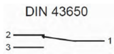
Fig. 16: Switch position under no-flow condition
