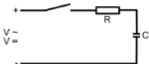
Fig. 29: Protective measure against capacitive loads
